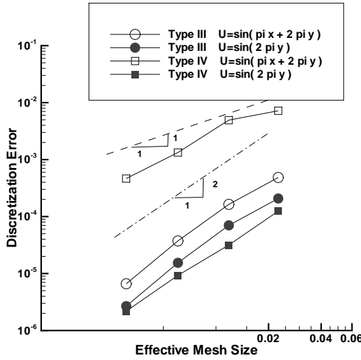
Figure 13. Convergence of discretization error ( L_1 norm) for node-centered FVD schemes on stretched irregular triangular grids with discontinuous metrics
