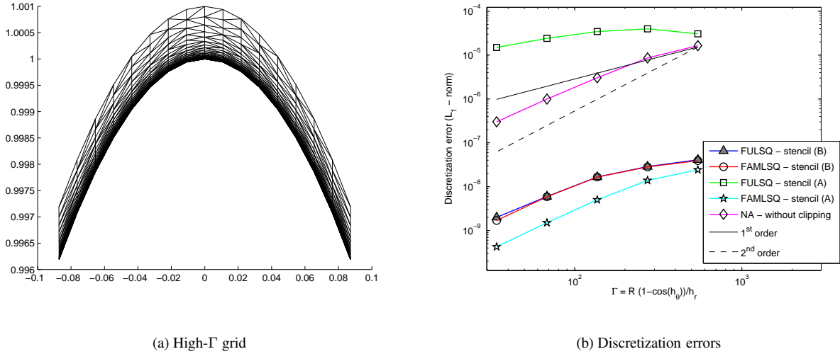
Figure 16. Cell-centered discretizations on high- \Gamma grid of type (III)
