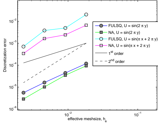
Figure 12. Convergence of discretization error ( L_1 norm) for cell-centered FVD schemes on stretched irregular triangular grids with discontinuous metrics
