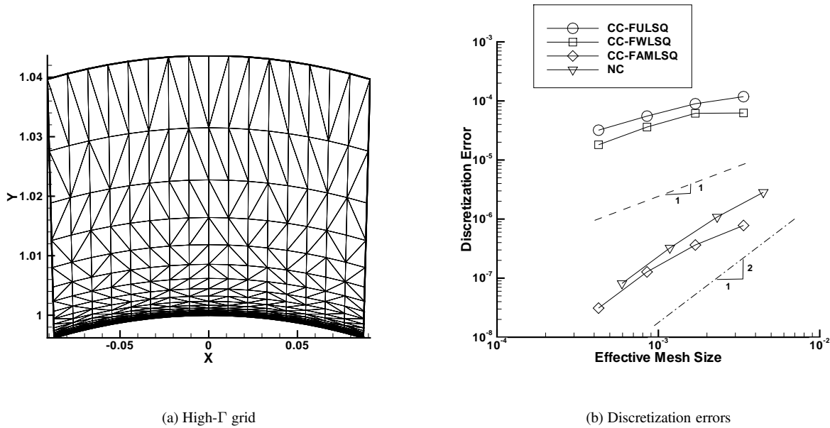
Figure 15. Comparison of cell-centered and node-centered discretizations on high- \Gamma grids of type (III)
