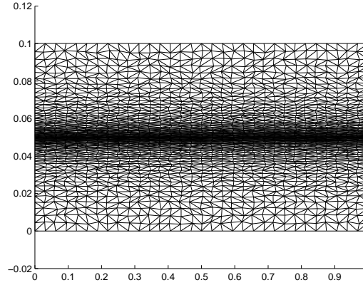
Figure 11. Random triangular stretched grid with 33 \times 65 nodes
